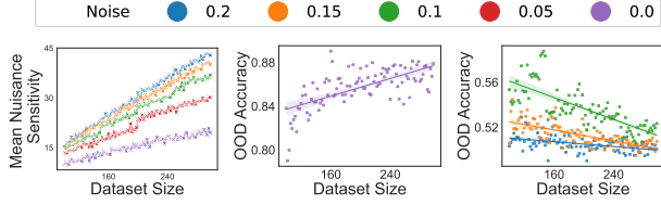
Figure 5. The left plot shows as the amount of label noise increases, nuisance sensitivity increases faster with larger dataset sizes. This leads to worse OOD accuracy, shown in the right plot. However, this phenomenon is not observed without label noise (middle plot).
