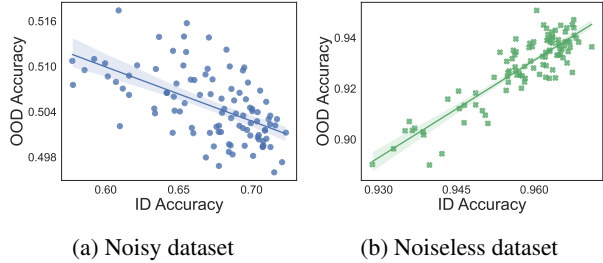
Figure 1. Accuracy-on-the-wrong-line behaviour in Noisy dataset vs. Accuracy-on-the-line behaviour in Noiseless dataset in linear setting. See Appendix A for a description of the setting.
