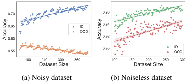
Figure 2. Same setting as Figure 1, increasing dataset size always increases ID accuracy irrespective of label noise, but decreases OOD accuracy in the presence of label noise.
