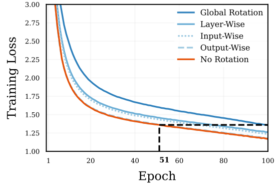
Figure 2: ViT/S (22M)
