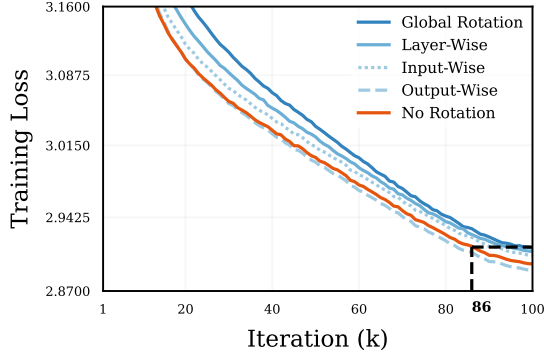
Figure 1: GPT2 (124M)
