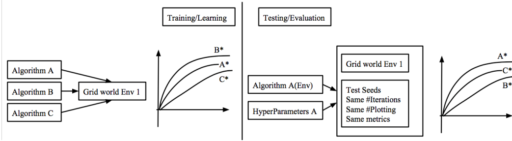
Figure 1: Overview of the evaluation pipeline: During the training phase, algorithms are compared against each with out-of-the box settings and weights of the learned model. At test time, the evaluation pipeline provides the ability to feed in a common choice of metric for evaluation and accessibility to the existing algorithms in a reproducible abstraction.
