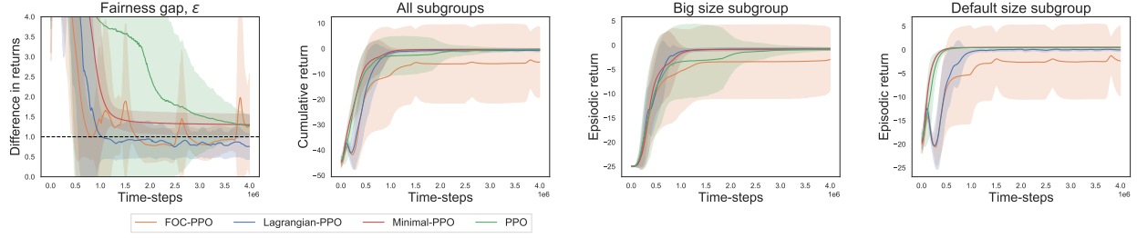
(b) Point-Navigation: Medium fairness threshold.
