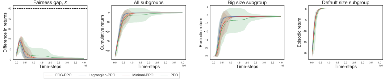
(a) Point-Navigation : High fairness threshold.
