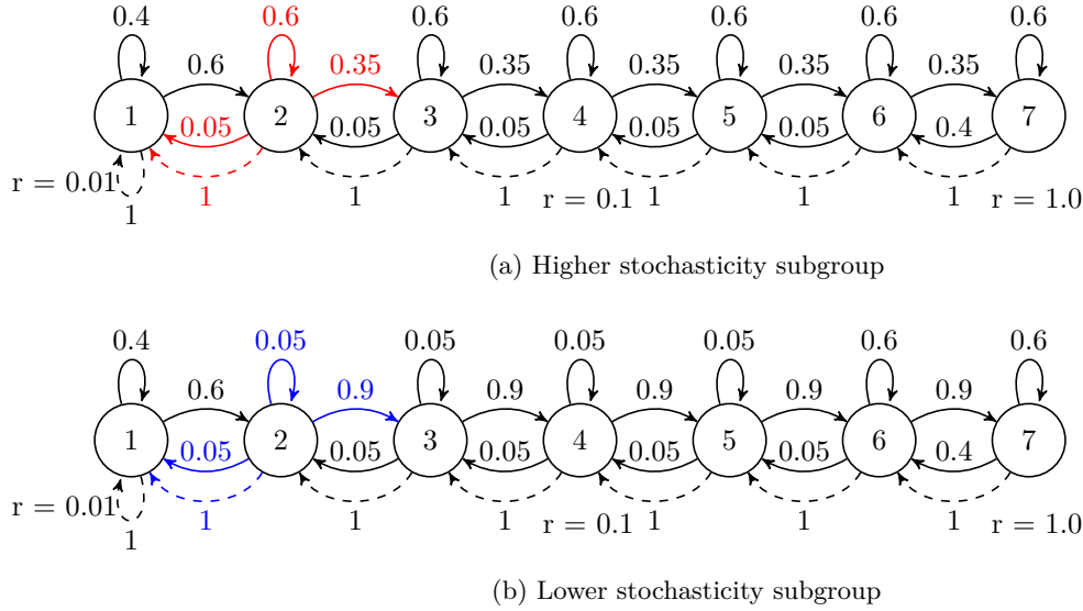
Figure 5: Description of the modified RiwerSwim environment. Figure 5a denotes the transition dynamics for the higher stochasticity subgroup, and Figure 5b denotes the transition dynamics for the other subgroup. The nodes in the graph denote the non-sensitive states and r denotes the reward function (that is same for both the subgroups). The solid arrows denote the transitions corresponding to taking the right action, and the dashed arrows denote left action. The number above arrows denotes the probability that action will result in the corresponding transition.
