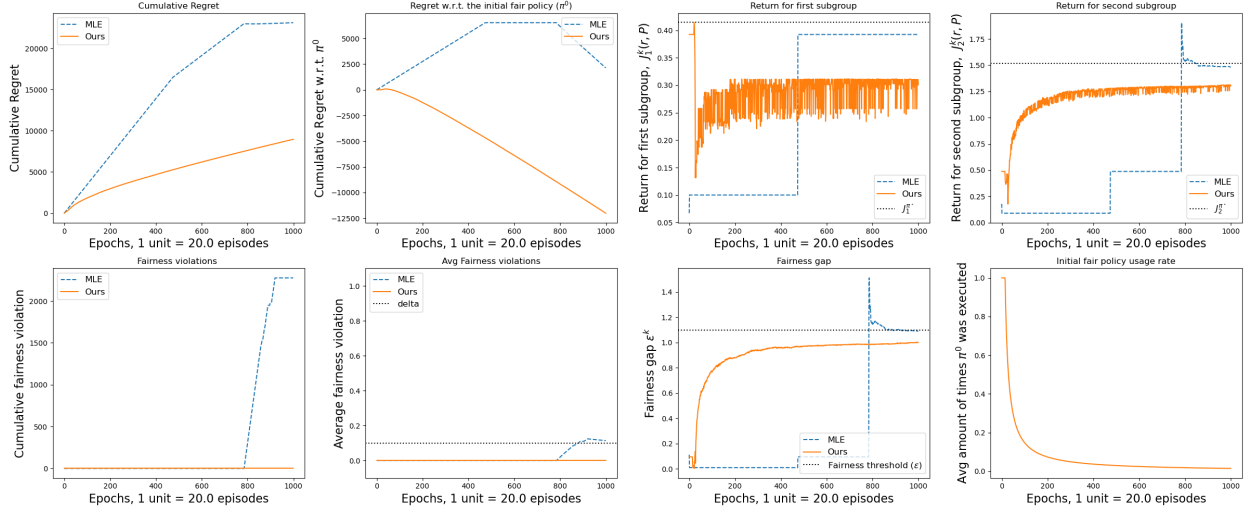
Figure 7: River swim environment with a starting \pi^0 with an inefficient exploration strategy, i.e., \pi^0 has very low probability of discovering the right most state ( B = 10^{-4} ).
