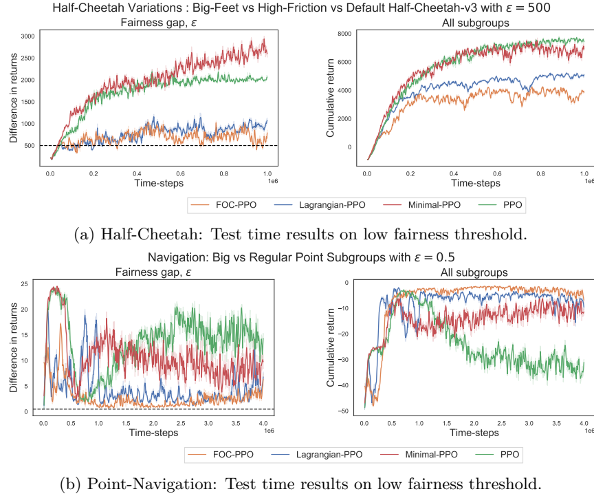
Figure 13: Test time performance plots for the Half-Cheetah and Point-Navigation environments with low \epsilon on 10 unseen environment instantiation with different random seeds. The first subplot in each row denotes the fairness gap (maximum of absolute difference of returns between subgroups) and the black dotted horizontal line denotes the specified acceptable fairness threshold ( \epsilon ). The second subplot in each row denotes the cumulative return for all subgroups. The x-axis denote the number of samples used during the learning. The solid colored lines represent the smoothed mean over 10 random seeds for different baselines (with weight=0.9) and the colored shaded regions represent the normal 95% confidence interval.
