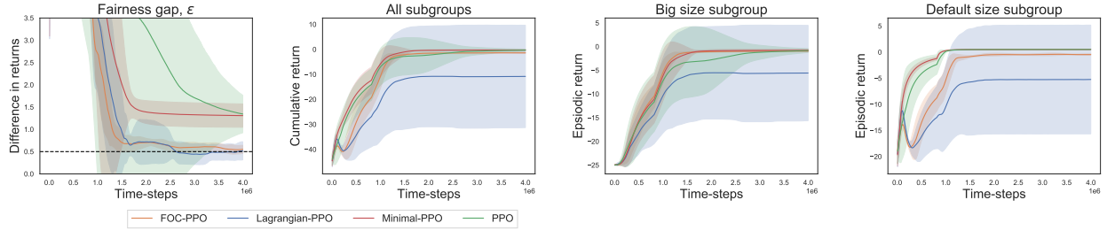
(c) Point-Navigation: Low fairness threshold.
