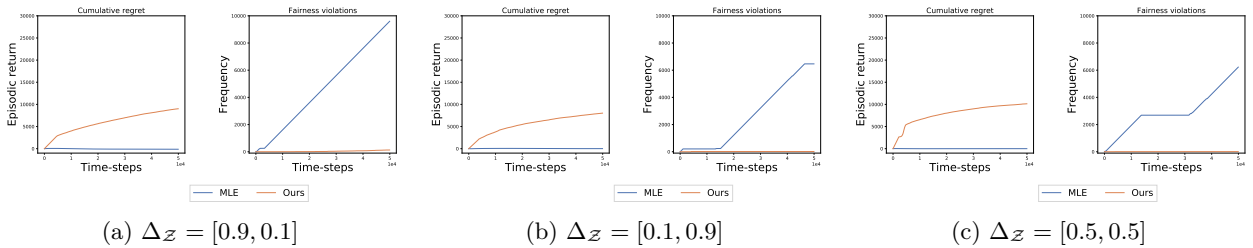
Figure 2: Regret and fairness violations on the credit landing environment for different underlying group distributions, where \Delta_{\mathcal{Z}} denotes [\Pr(\text{high}), \Pr(\text{low})] . In all the scenarios, our proposed approach achieves sub-linear regret and close to zero fairness violations.
