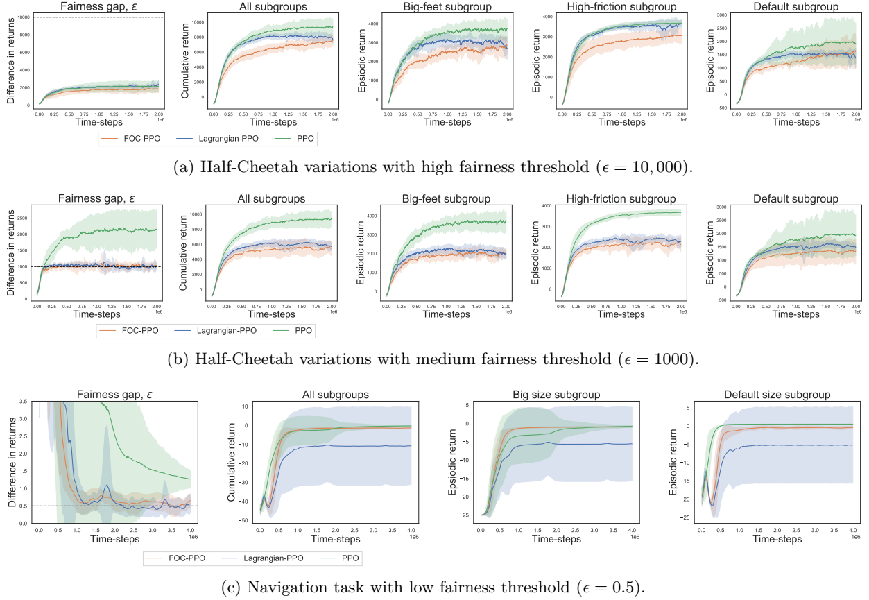
Figure 4: Learning curves for different environments with different fairness thresholds. The first subplot in each row denotes the fairness gap (maximum of absolute difference of returns between subgroups) and the black dotted horizontal line denotes the specified acceptable fairness threshold ( \epsilon ). The second subplot in each row denotes the cumulative return for all subgroups, and the rest of the subplots in the row denote the subgroup specific returns. The x-axis denote the number of samples used during the learning. The solid colored lines represent the smoothed mean over 10 random seeds for different baselines (with weight=0.9) and the colored shaded regions represent the normal 95% confidence interval. Plots for running mean over the last 100 episodes are included in Appendix G.
