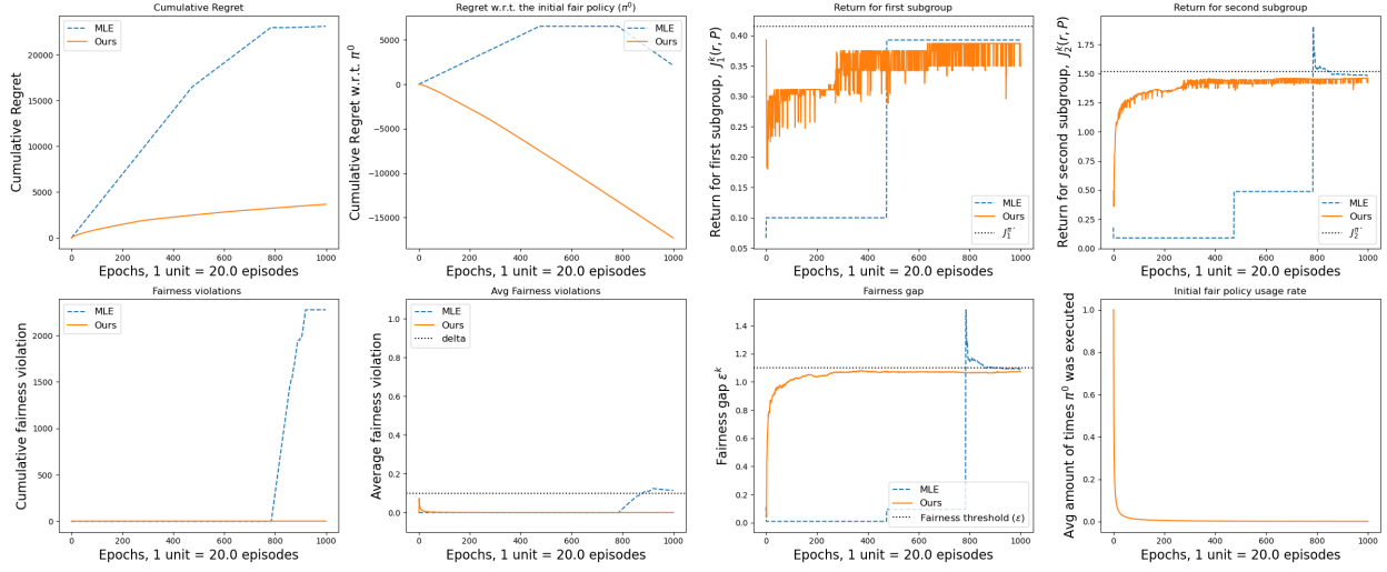
Figure 6: River swim environment with a starting \pi^0 with an inefficient exploration strategy, i.e., \pi^0 has very low probability of discovering the right most state (Fine-tuned B hyper-parameter).
