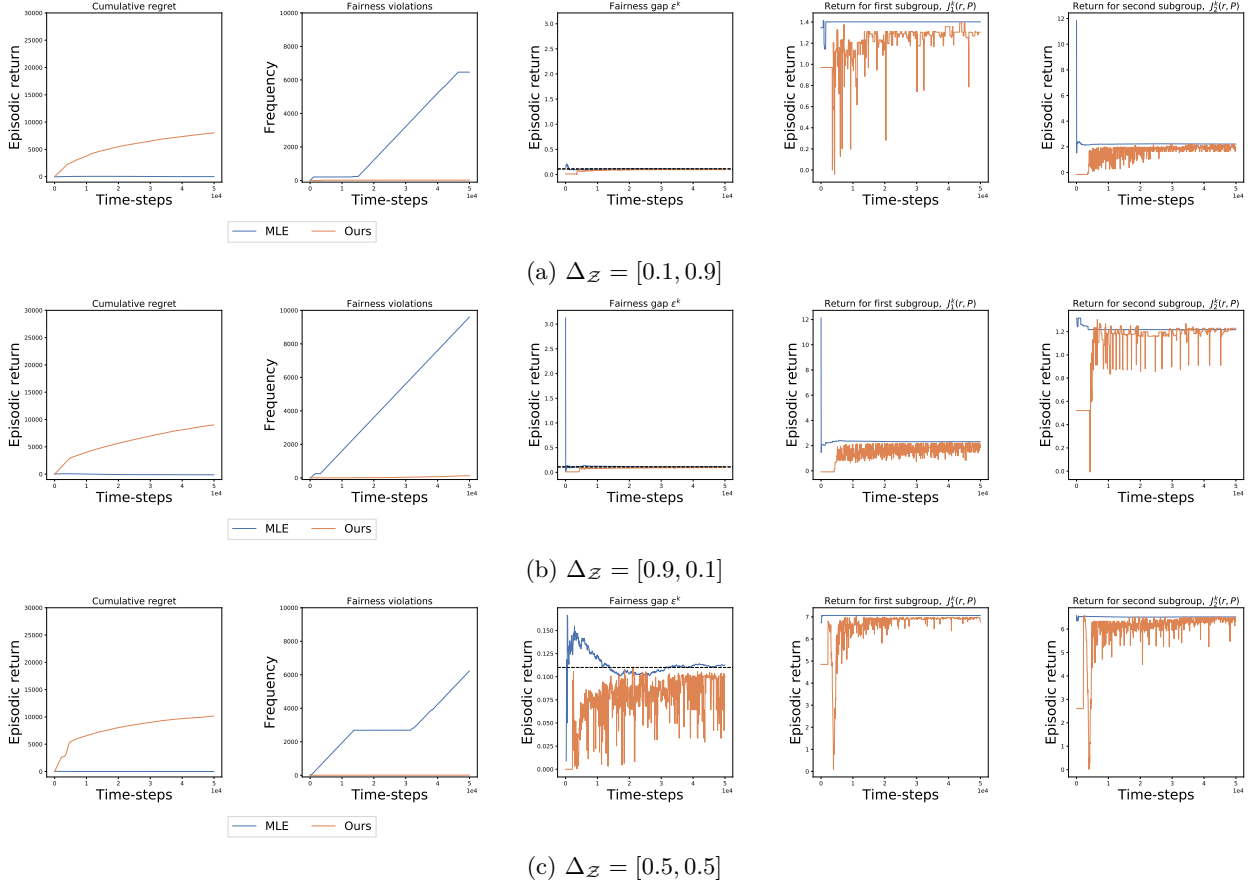
Figure 8: Learning curves for the credit lending task with different \Delta_{\mathcal{Z}} . The subplots in each row denote the following (from left to right): cumulative regret, number of fairness violations, fairness gap between the groups, return of group high , return of group low . The x-axis denote the number of samples used during the learning.
