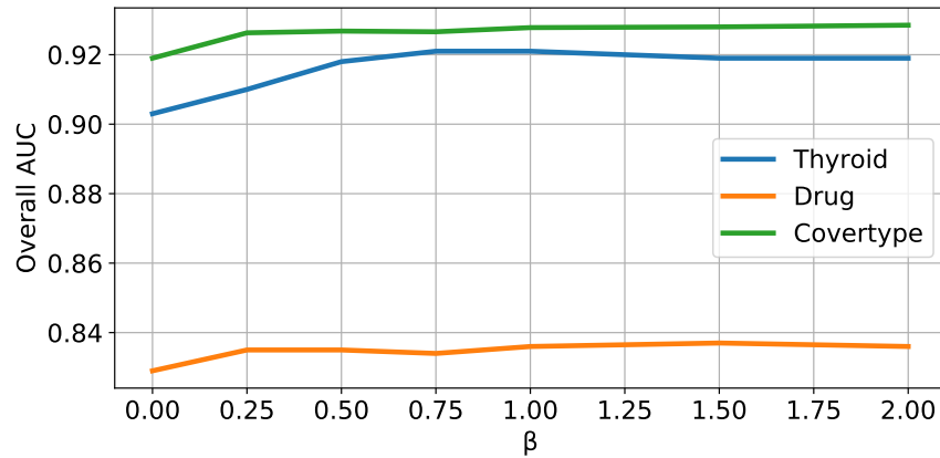
Figure 6: Overall AUC across different values of \beta using three tabular datasets. ( \beta = 0 represents SPADE without self-supervised learning.)
