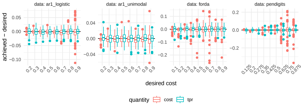
Figure 4.2: The boxplot of the deviance in the achieved v.s. desired cost (varying from 0.1 to 0.9) and TPR (0.9) over the 100 repeated experiments under the setup of Figure 4.1 , grouped by the desired cost (x-axis).
