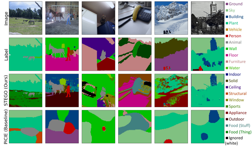
Figure 9: STEGO failure cases.
