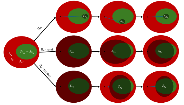
Figure 1: A visualization of searching for a goal with a monotonic specification, \Pi_m , and a non-monotonic specification, \Pi_n . The set of goal states is shown in green and denoted by S_{\Pi_m} , which is equal to S_{\Pi_n} . The set of non-goal states is shown in red and denoted by S_{\Pi'} . The black dot represents the start state and is denoted by s_0 . The set of states represented by an assignment is shown in transparent black and is denoted S_{A_i} . The blue arrow represents a path to an assignment. The monotonic specification does not need to be specialized since all candidate states are goal states. On the other hand, the non-monotonic specification can produce assignments that can be specialized randomly or with a conflict-driven approach. This conflict-driven approach can lead to finding shorter paths with less time.
