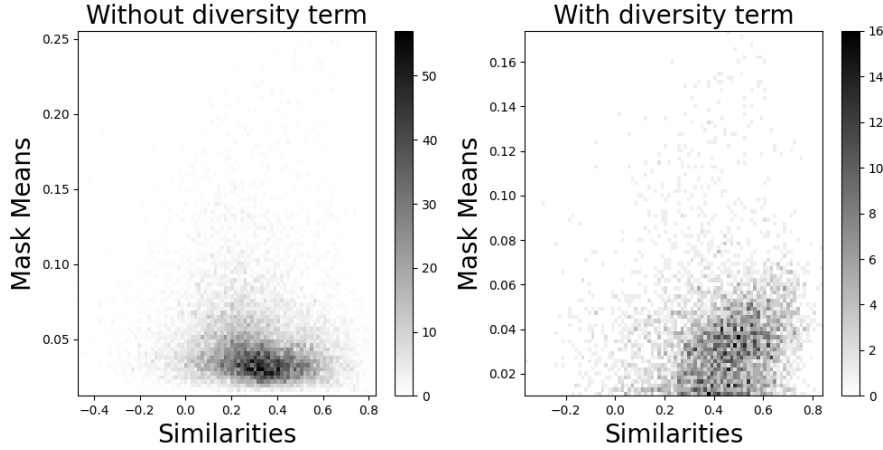
Figure 10: Audio-text similarity after audio masking, without the diversity term (left), with the diversity term (right).
