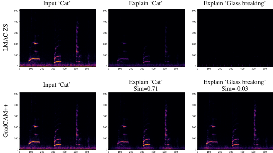
Figure 4: Qualitative Comparisons of Explanations given by LMAC-ZS, and GradCAM++, for two different classes. We see that LMAC-ZS shuts-off the explanation depending on the similarity of the given prompt with the input audio, whereas GradCAM++ remains insensitive to the class label.
