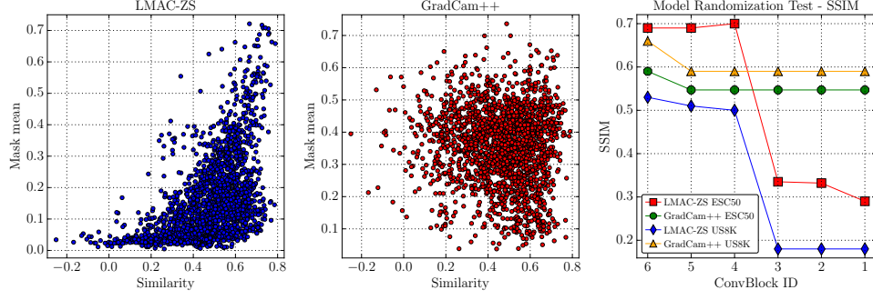
Figure 3: (left) Mask-Mean vs Similarity for LMAC-ZS, (middle) Mask-Mean vs Similarity for GradCam++, (right) Model Randomization Test for LMAC-ZS and GradCam++.
