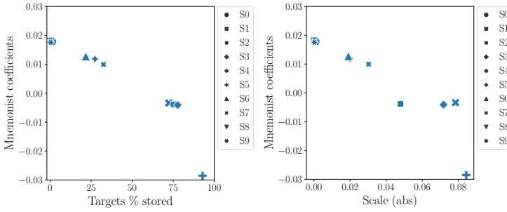
Figure 7: Coefficients of the interpretable model in Mnemonist as a function of number of target points stored in each superparameter across 1,000 released models (left) and scale of storing target points in each superparameters after 1 step. Mnemonist coefficients are aligned with training dynamics such that it can detect important and redundant superparameters.
