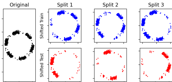
Figure 1: VV systematically thins the distribution in a certain region for training (top row) and then evaluates whether the generated samples in the thinned region after reweighting matches the complementary held-out test dataset (bottom row). In contrast, standard evaluations will seek to match the macro properties (e.g., mean) of this distribution which emphasizes the regions of thick support. The original data (left) illustrates both thick support regions (i.e., areas with many samples) and thin support regions (i.e., areas with very few samples).
