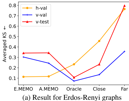
Figure 4: On both Erdos-Renyi and Comm20 datasets, our proposed vertical validation approach (VV) can select the best model for generating in thin support as shown by the test line, whereas the standard train-test splitting (CV) tends to favor memorization despite poor generalization to the thin support regions. Note that for CV, the oracle distribution seems worse than memorization because oracle is generating from the true distribution rather than the shifted training distribution—thus it appears to CV that memorizing is actually a better option. This phenomena does not happen in our validation approach because we aim to find a model that generalizes to the thin support well. This also showcases that our approach is better able to detect memorization than the standard train-test split validation.
