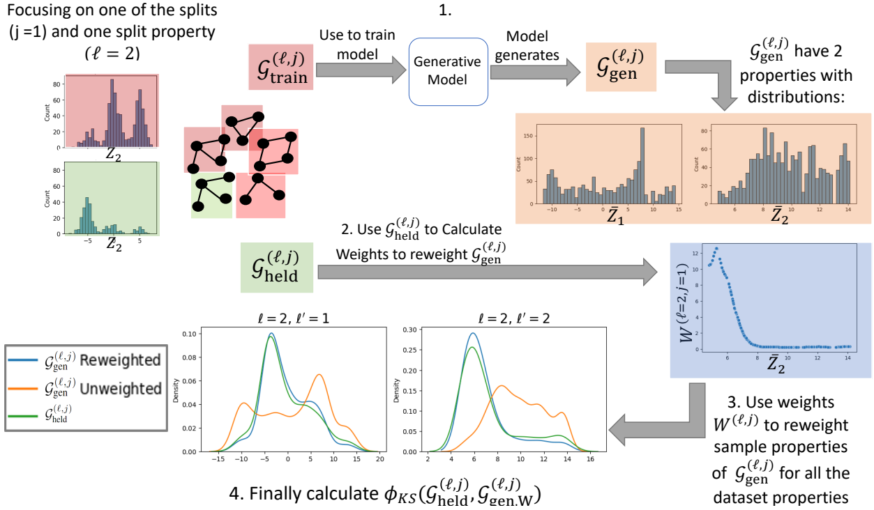
Figure 8: (1) using \mathcal{G}_{\text{train}}^{(\ell,j)} we train a generative model which then generates \mathcal{G}_{\text{gen}}^{(\ell,j)} . For the generated dataset we can compute the properties of interest ( \bar{Z}_1 and \bar{Z}_2 ). (2) Use \mathcal{G}_{\text{hold}}^{(\ell,j)} to calculate the weights W^{(\ell,j)} which will then be used in (3) to re-weight the samples in \mathcal{G}_{\text{gen}}^{(\ell,j)} by applying those weights to the calculated properties. The Density figures above show the difference in distribution between the re-weighted and un-weighted versions of the generated data as well as how they compare to the held-out part of the data. (4) Finally we can compute the KS statistic between the weighted \mathcal{G}_{\text{gen}}^{(\ell,j)} and \mathcal{G}_{\text{hold}}^{(\ell,j)} as detailed in Equation 6.
