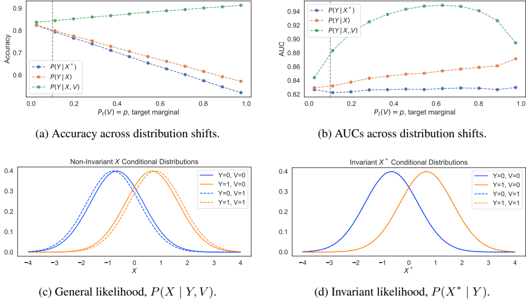
Figure 3: Simulation study described in Section 3. Panel (a) compares the predictive accuracy of the models P_s(Y|X) , P_s(Y|X^*) and P_s(Y|X, V) as a function of the target marginal P_t(V) = p , with source P_s(V) = .1 . Only P_s(Y|X, V) does not degrade in accuracy as P_t(V) shifts further away from P_s(V) . Panel (b) compares the predictive AUC of the same three models. Note that the predictor using X^* , P_s(Y|X^*) does achieve invariance in AUC across shifts, but not accuracy (or likelihood), and cannot make use of information about Y from V . Panel (c) depicts the four likelihood models (one for each combination of Y and V ) — note that V = 1 further separates the conditional distributions, making separation easier (hence the AUC goes up in Panel (b) as p increases). Panel (d) depicts a P(X^*|Y, V) , which is the same across values of V (unlike P(X|Y, V) in Panel (c)). The overall key takeaway is the robustness of P_s(Y|X, V) , i.e. the model conditioning on both V and X versus the lack of robustness in models conditioning only on X or X^* in terms of predictive accuracy in Panel (a) (even when their AUC is robust across shifts, Panel (b)).
