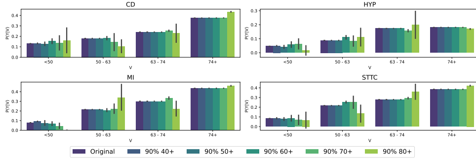
Figure 4: Validation of shifts for V=Age . For each of the 4 superdiagnostics (subplots), we show P(Y|V_A = v) per v \in \{< 50, 50 - 63, 63 - 74, 74+\} (leftmost group of bars in subplot to rightmost group of bars in subplot) for the original, unshifted test set (dark purple) and the shifts introduced in Section A.2.1. Equal height of bars inside each group of bars is indicative for constant P(Y|V) across evaluation sets.
